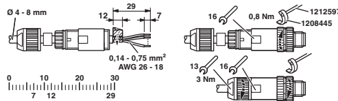
Functional drawing
